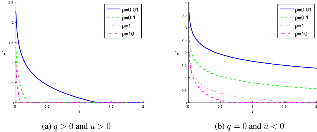
FIGURE 4. The optimal threshold level A^* with various values of coefficients of absolute risk aversion \rho : (a) q = 0.1 and \bar{u} = 0.5 ( c = 1, \sigma = 1, \eta_- = 2, \eta_+ = 1, \lambda = 1 ) and (b) q = 0 and \bar{u} = -1.5 ( c = -1, \sigma = 1, \eta_- = 2, \eta_+ = 1, \lambda = 1 ).
